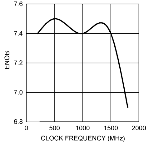
ENOB vs. CLOCK FREQUENCY
